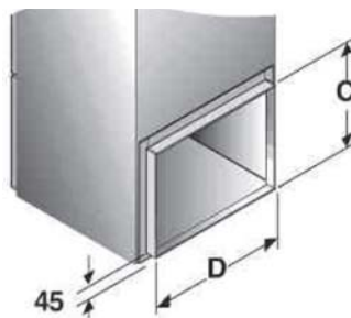
Rear Inlet
