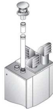
Fan assisted flue through roof (type B22) without combustion air pipe
