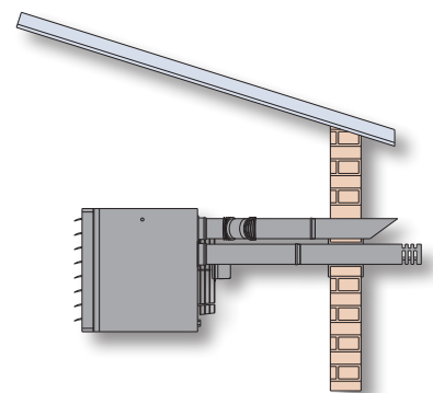
Separate combustion air and flue pipes (type C12) for applications where wall thickness 350mm. Flue and air intake to be offset
